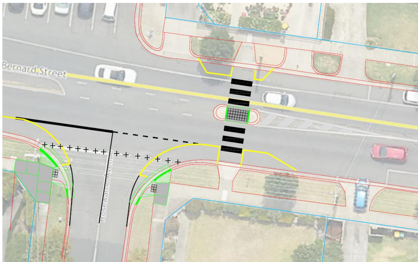
Figure 1: Depiction of proposed pedestrian crossing upgrade and additional traffic treatments to be installed outside 41 Bernard Street, Cheltenham.
